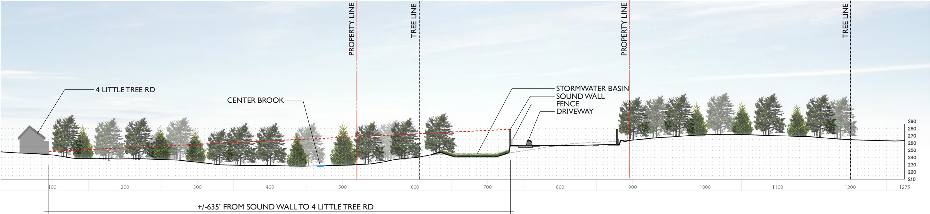
SECTION B-B
